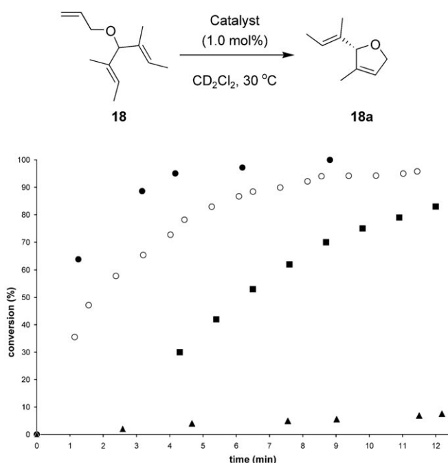
Figure 3. Ring-closing metathesis of 18 using catalysts 4 (●), 16-Pr (○), 16-Bn (■) and 1a (▲). Conversions determined by 1 H NMR spectrum of reaction mixture.
