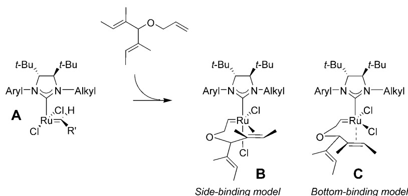
Figure 4. Possible intermediates in the cyclizations of meso -triene 18 with catalysts bearing C_1 -symmetrical NHC ligands.
