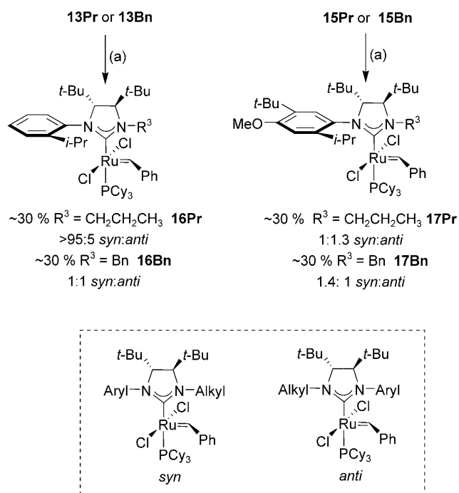
Scheme 2. Synthesis of new catalysts; reaction conditions: (a) (\text{CF}_3)_2\text{CH}_3\text{COK} (1.5 equiv.), \text{PhMe} then (\text{PCy}_3)_2\text{Cl}_2\text{Ru}=\text{CHPh} 3 (1 equiv.), 60^\circ\text{C} , 3 h. Only the major syn rotational isomer is shown above.
