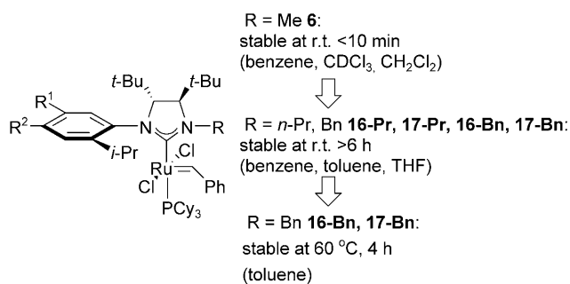
Figure 2. Improved thermal and solution stability through variation of the N-alkyl group of the NHC ligand.
