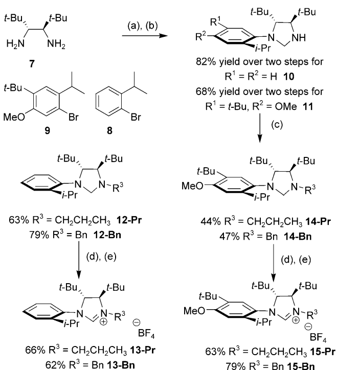
Scheme 1. Synthesis of new N-heterocyclic carbene ligands via N-alkylation; reaction conditions: (a) \text{Pd}_2(\text{dba})_3 (5 mol%), (t\text{-Bu})_3\text{PHBF}_4 (20 mol%), \text{NaO}-t\text{-Bu} (4 equiv.), 8 or 9 , \text{PhMe} , 100^\circ\text{C} , 24 h; (b) paraformaldehyde (1 equiv.), \text{CH}_2\text{Cl}_2 , 21^\circ\text{C} , 24 h; (c) \text{R}^3\text{CH}_2\text{Br} , \text{K}_2\text{CO}_3 , acetone, 100^\circ\text{C} , sealed tube, 12–48 h; (d) \text{I}_2 , \text{NaHCO}_3 , \text{CH}_2\text{Cl}_2 , 21^\circ\text{C} , 24 h; (e) \text{NaBF}_4 , \text{Na}_2\text{SO}_3 , 21^\circ\text{C} .
